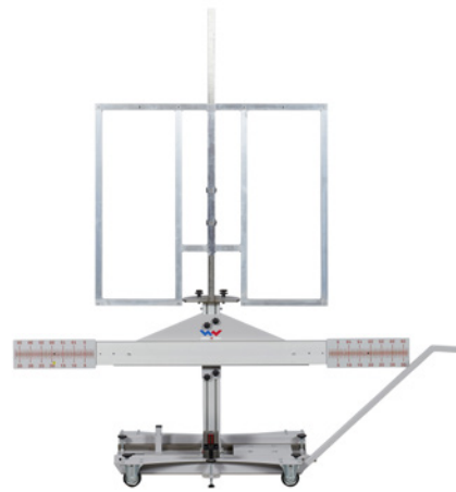
Extension camera calibration Transporter & Car* Art. no. WW01000663
